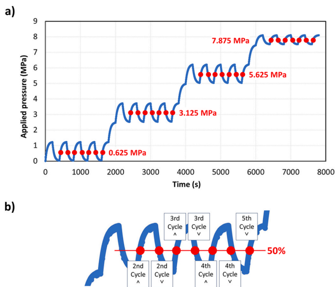
Fig. 2. a) Compression cycles and the mean value for each of them; b) Choice of values in the generic range of the mechanical compression profile applied to the GDL.
