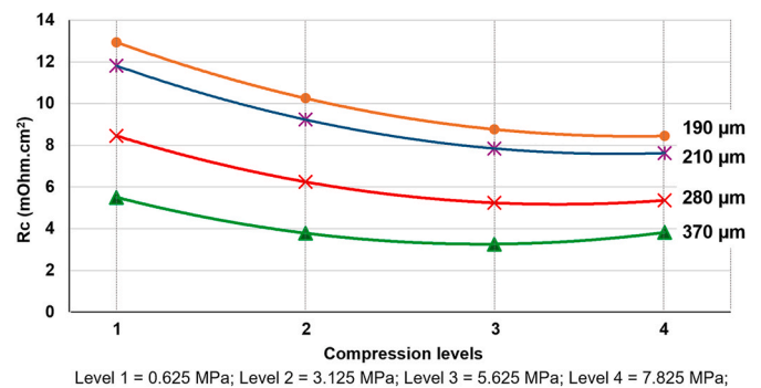
Fig. 7. – R c as a function of the mechanical compression for each thickness level.
