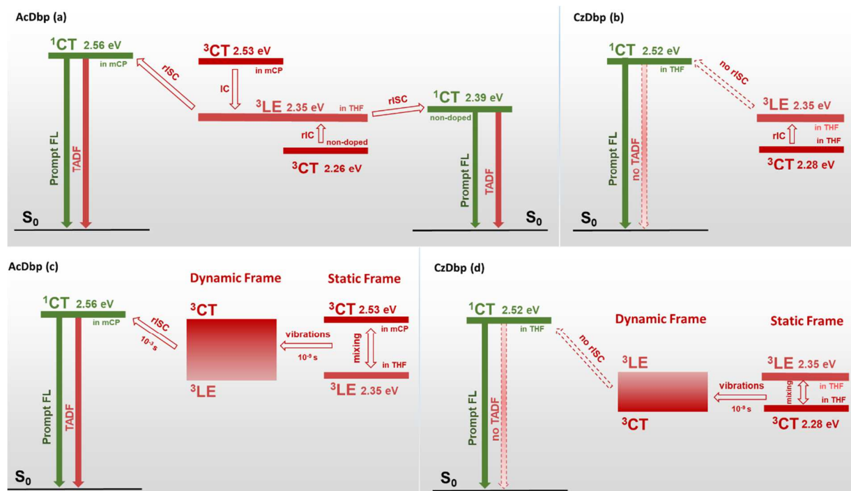
Fig. 9. Diagrams of excited states energies of AcDbp (a) and CzDbp (b); diagrams illustrating the “dynamic” mechanism of mixing between LE and CT states through dihedral vibrations [56,57,58] in AcDbp (c) and CzDbp (d)
