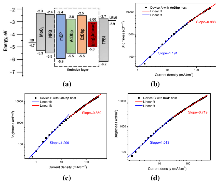
Fig. 7. Equilibrium energy diagram (a) of devices A-C. IP^{PE} and EA^{PE} values of solid samples of AcDdbp and CzDdbp were taken for the design of the device structures (Table 2). Linear fits to current density versus brightness plots for devices A-C (b-d).
