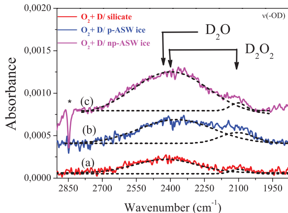
FIG. 4. RAIRS spectra of D_2O and D_2O_2 ices formed after the exposure of 1 ML of solid O_2 and 2.0 ML of D atoms on different substrates held at 10 K: (a) amorphous silicate, (b) p-ASW ice, and (c) np-ASW ice. The dashed curves are the Gaussian fits. (The star at 2850\text{ cm}^{-1} is an impurity.)
