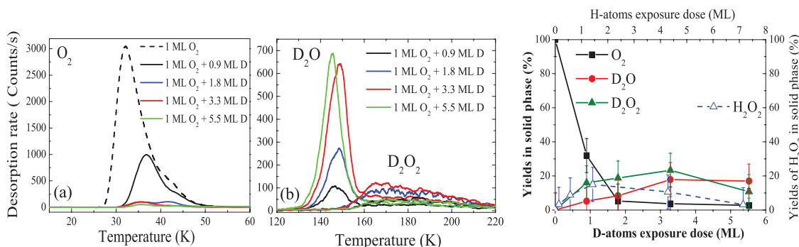
FIG. 3. (Left panel) (a) and (b) the desorption rates of O_2 , D_2O , and D_2O_2 species as a function of D-atom exposure doses (0, 0.9 ML, 1.8 ML, 3.3 ML, and 5.5 ML) on 1 ML coverage of O_2 ice film deposited on the silicate surface held at 10 K. (Right panel) The evolution of the yields (in %) of O_2 , D_2O , and D_2O_2 species present on the surface of the silicate as a function of D-atom exposure doses. The blue dashed line is the yields (in %) of H_2O_2 molecules present on the surface of the silicate as a function of H-atom exposure doses. The uncertainties of the measurements are marked by the errors bars.
