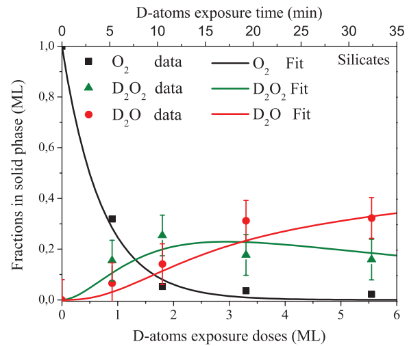
FIG. 8. (Full triangles, circles, and squares) The amount (in ML) of O 2 , D 2 O, and D 2 O 2 species present on the surface as a function of D-atoms exposure doses on 1 ML coverage of O 2 ice deposited on the silicate sample at 10 K. (Solid lines) The fits of O 2 , D 2 O, and D 2 O 2 obtained from the model with \alpha = 0.69 , k = 1 , k_1 = 0.09 , \mu = 1 , \mu_1 = 0.14 , and the fraction of D 2 O desorbed from upon formation by the exothermic OD + D reaction is e_v = 86\% . The uncertainties are given by the errors bars which are equal to 0.08 for D 2 O and 0.1 for D 2 O 2 .
